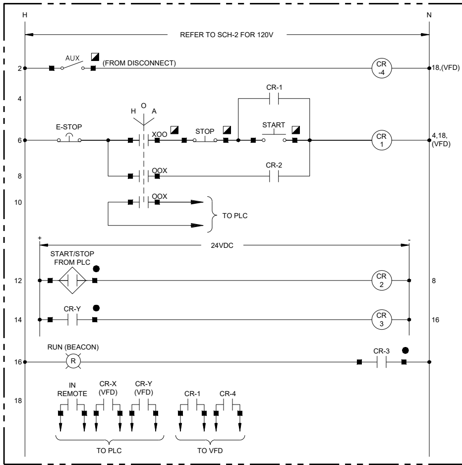
TEST PUMP SCHEMATIC 1 -
